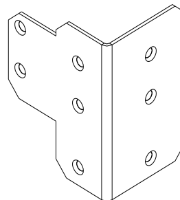
(#18-A) Right Front Bottom Corner Protection x 1 PC
