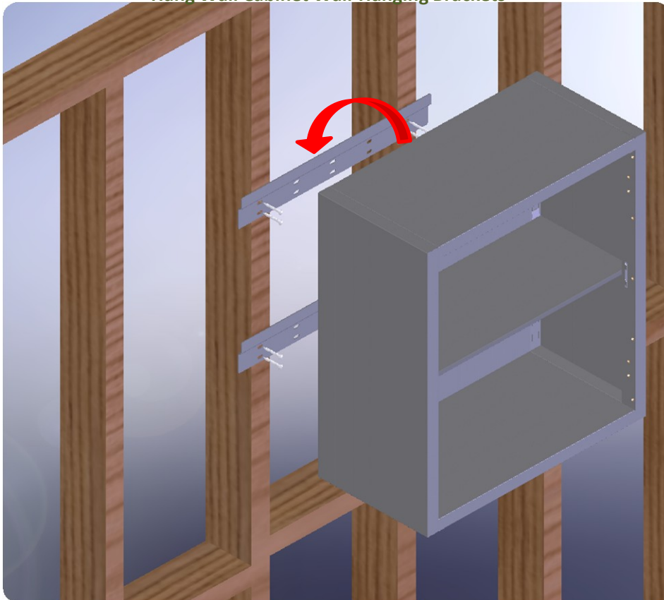
Hang Wall Cabinet Wall-Hanging Brackets
