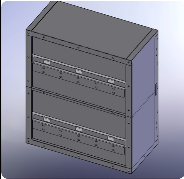
Back Panel View of Wall Cabinet shows 6 flat hooks that allow the Cabinet to hang on two Wallhanging Brackets.
