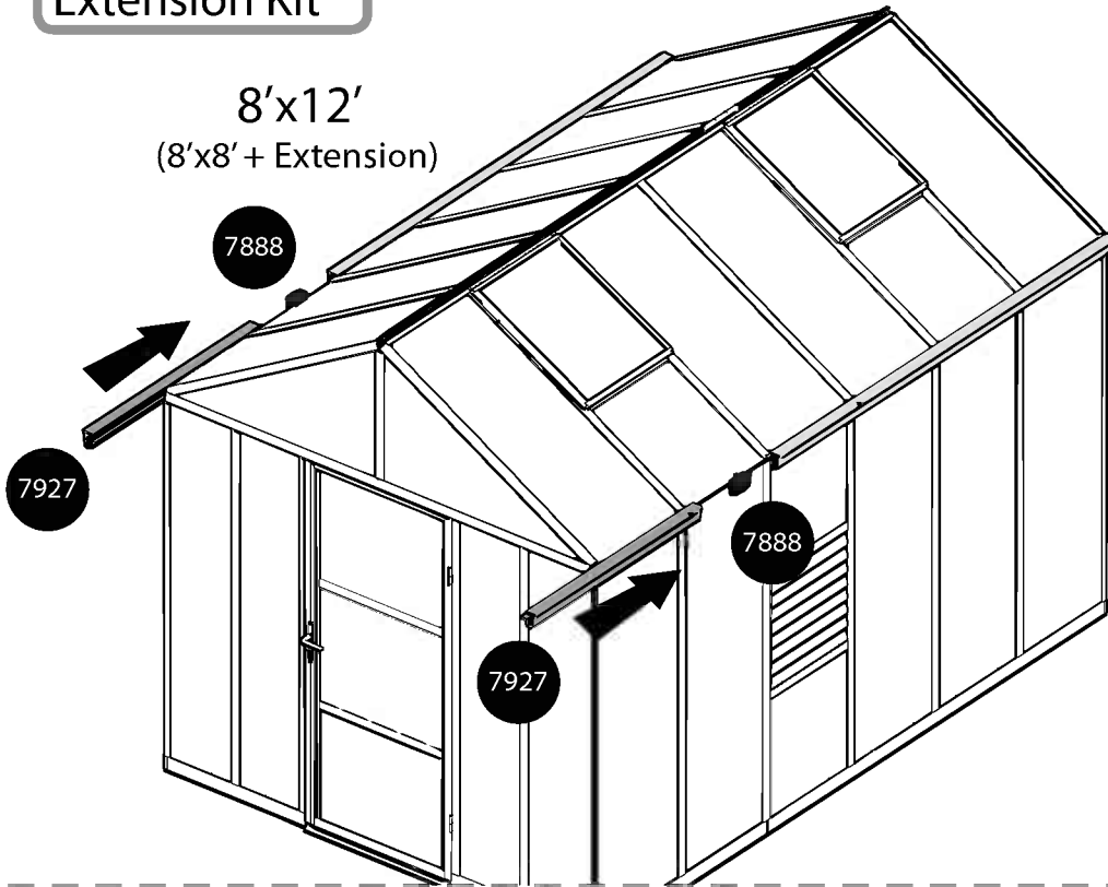
Extension Kit
