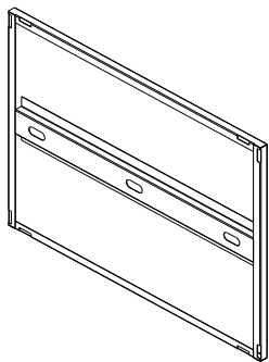
(#9) MIDDLE SHELF x 1 PC
